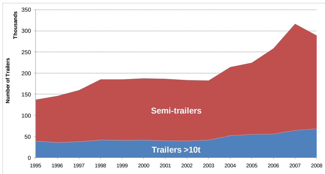
Figure 2–29: EU27 trailer registrations by type (with trailers &lt;10t removed), 1995-2008 (Eurostat, 2010)
