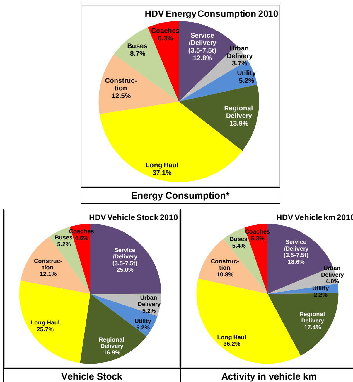
Figure 4–3: Estimated breakdown of the EU HDV energy consumption, activity and vehicle parc by mission profile for 2010
