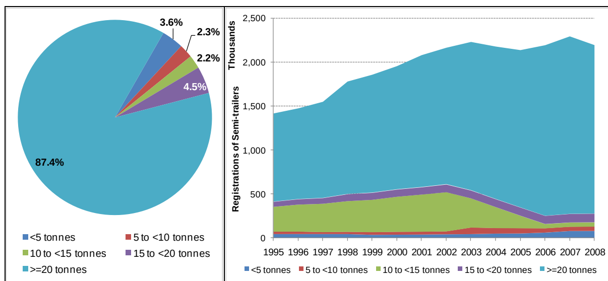
Figure 2–50: EU27 Semi-trailer parc, by load capacity (number), timeseries 1995 to 2008 and 2008 split
