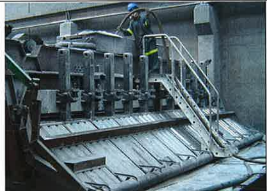
Figure 2 . Portable point feeder stair and use.
