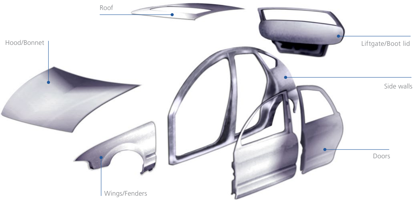
Figure 11: Aluminium hang-on parts
