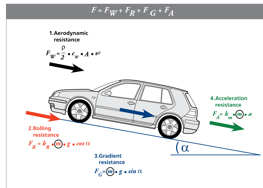
Figure 3: Resisting forces
